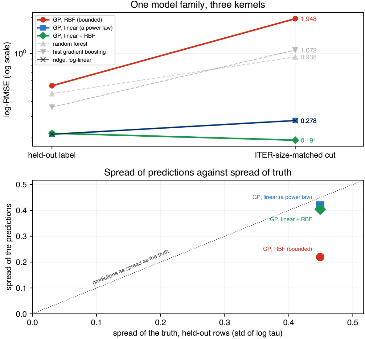
Figure 4: One model family, three kernels. Gaussian processes with a radial-basis-function (RBF) kernel, a linear (dot-product) kernel, and their sum. Top: log-RMSE on a held-out label and at the ITER-size-matched cut. The kernels differ in whether they permit a trend that continues at long range; adding the linear component also enlarges the function class. Bottom: spread of the predictions against spread of the truth on the held-out rows. A model whose posterior has reverted to its prior mean predicts nearly the same value everywhere, so its spread sits near zero however good its in-range fit was: the same failure a tree ensemble shows when it cannot exceed its largest training target, reached by a different route.
