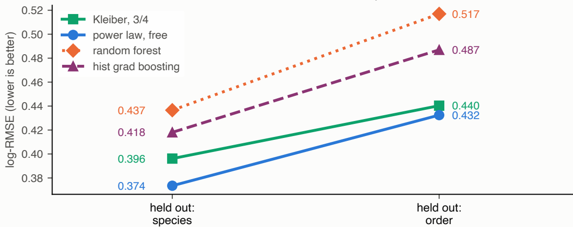
Kleiber's law under both splits
