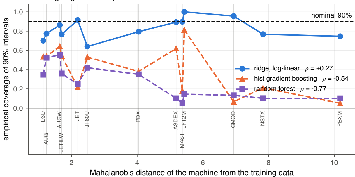
Coverage against extrapolation distance
