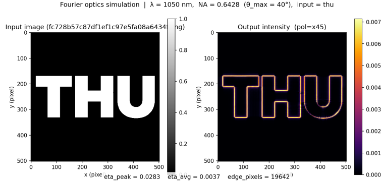
Figure 3: Image-domain validation for the leading 1050 nm second-order result. The response-level agreement translates into practical edge-enhancement behavior rather than remaining a numerical score gain only.
