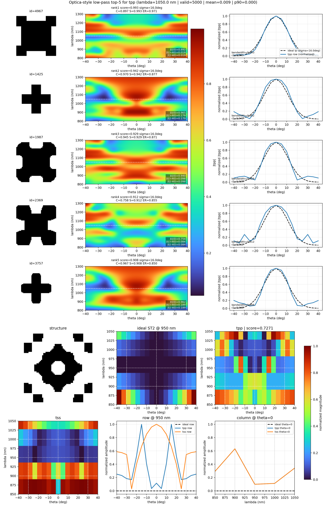
Figure 5: Generalization beyond second-order differentiation. Left: low-pass target at 1050 nm. Right: top spatiotemporal candidate at 950 nm from the wavelength-angle window ranking pipeline.
