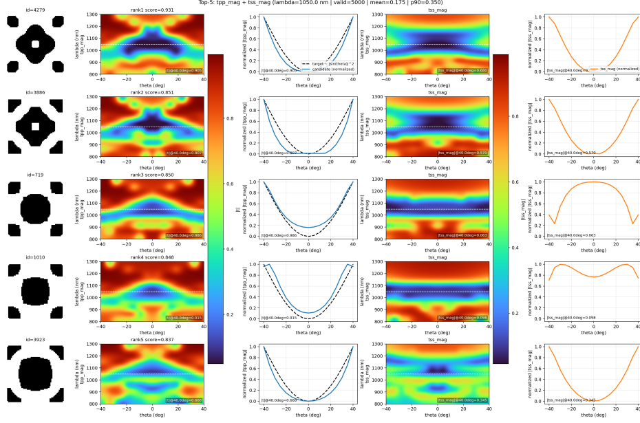
Figure 2: Top ranked second-order candidates at 1050 nm. The ranking overview visualizes the concentration of operator-like responses that motivates task-aware simulation-based reranking.
