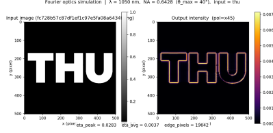
Figure 2: Image-domain validation for the leading 1050 nm second-order result. The response-level agreement translates into practical edge-enhancement behavior rather than remaining a numerical score gain only.
