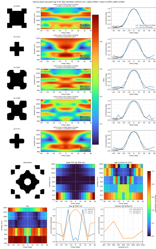
Figure 4: Generalization beyond second-order differentiation. Left: low-pass target at 1050 nm. Right: top spatiotemporal candidate at 950 nm from the wavelength-angle window ranking pipeline.
