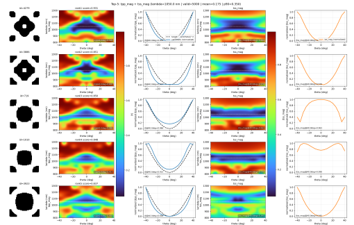
Figure 1: Top ranked second-order candidates at 1050 nm. The ranking overview visualizes the concentration of operator-like responses that motivates task-aware simulation-based reranking.
