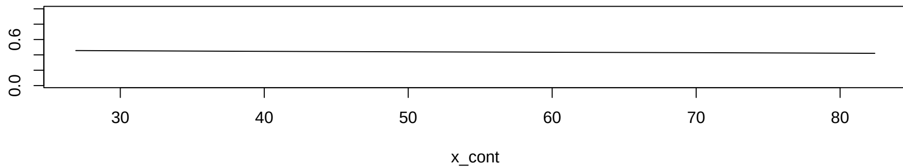
Conditional Distribution
