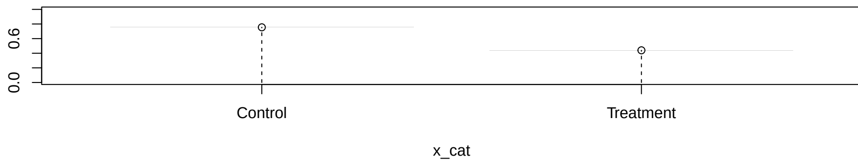
Conditional Distribution
