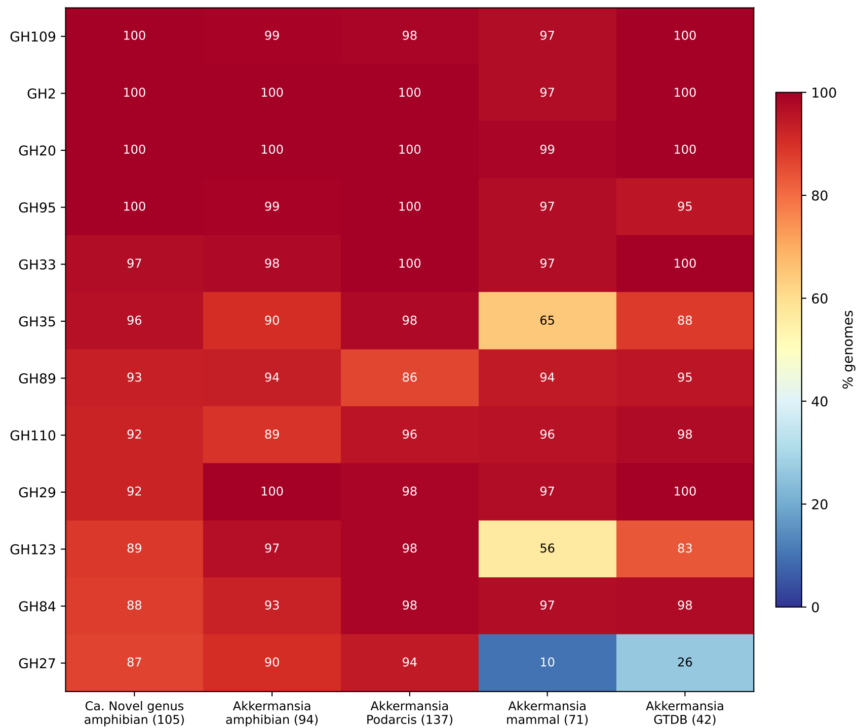
Mucin-degradation machinery is conserved across all gut-associated Akkermansiaceae
