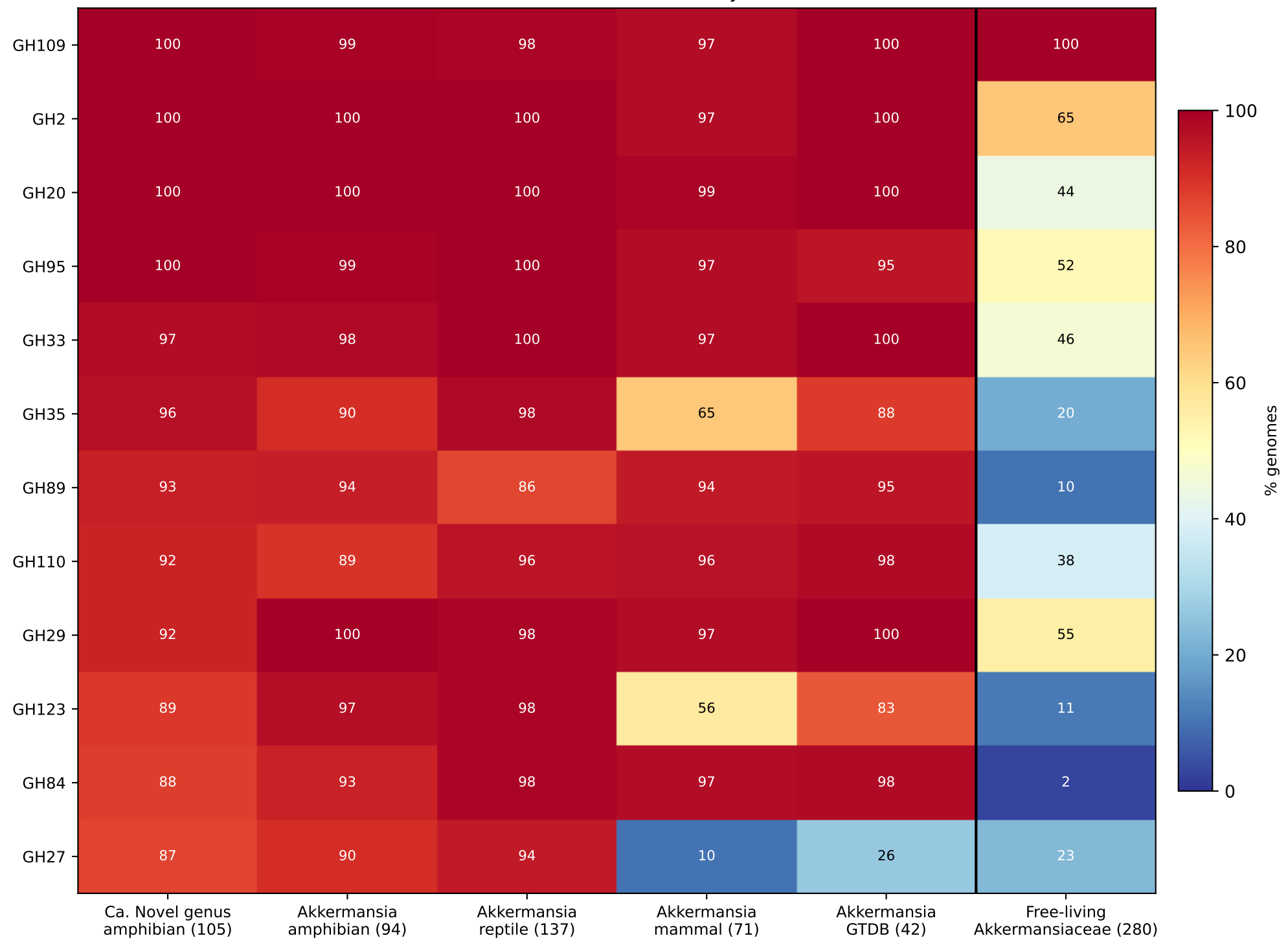
Prevalence of mucin-associated CAZyme families
