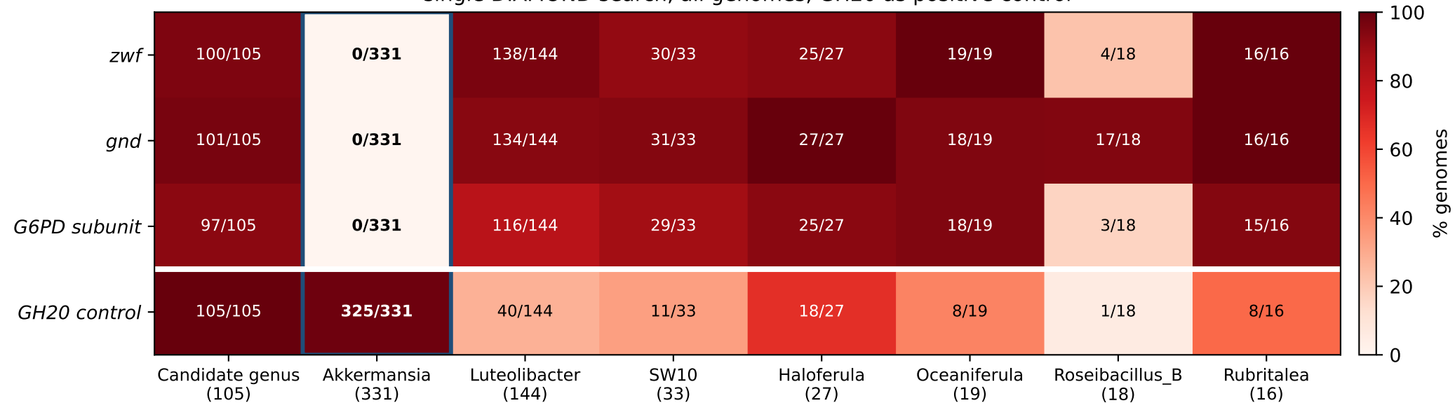
Oxidative pentose phosphate pathway across Akkermansiaceae single DIAMOND search, all genomes, GH20 as positive control
