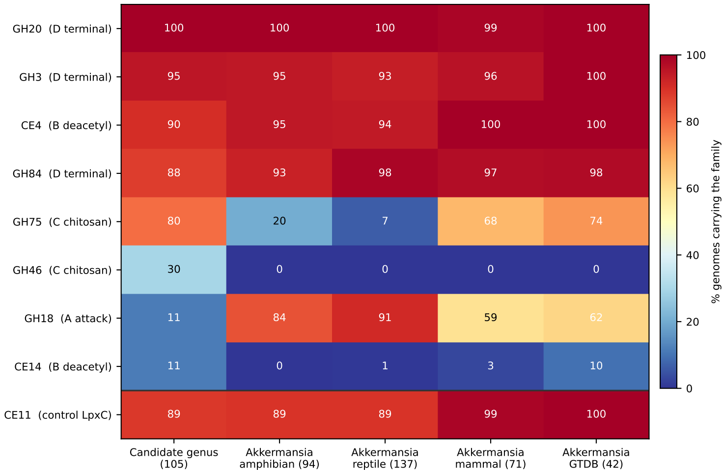
Prevalence of chitin-related CAZyme families across the candidate genus and Akkermansia
