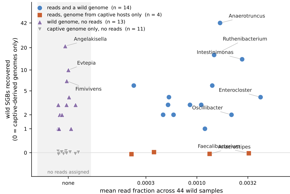
C Read abundance does not determine which lineages were recovered as genomes
