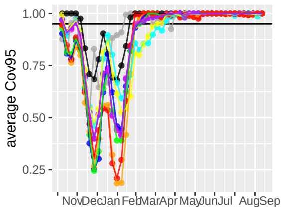
95% coverage (4 week)
