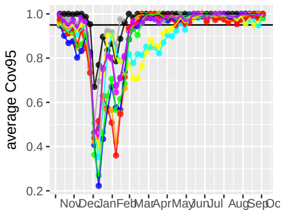
95% coverage (1 week)
