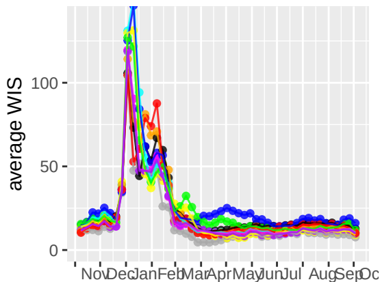
95% coverage (1 week)
