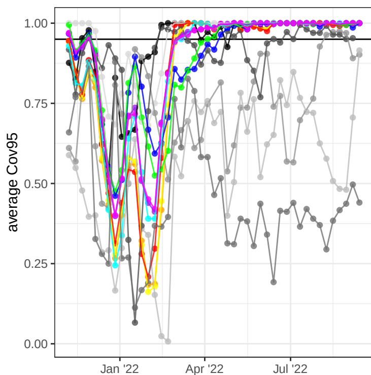
95% coverage (4 week)
