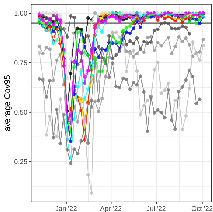
95% coverage (1 week)
