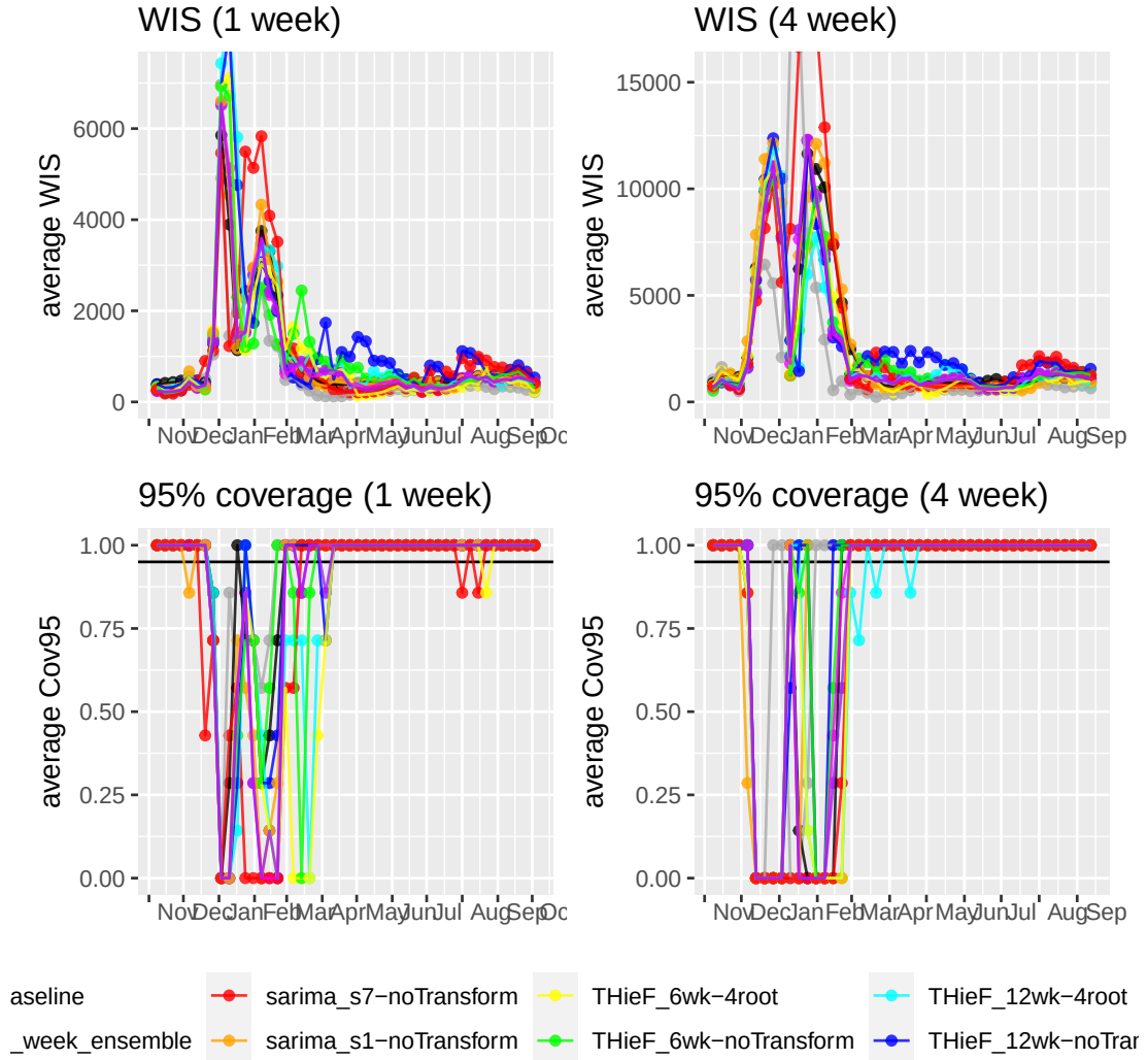
Figure 3.5. Average h-week ahead WIS and 95% PI coverage plotted by forecast week during the testing phase for each model for U.S. national
