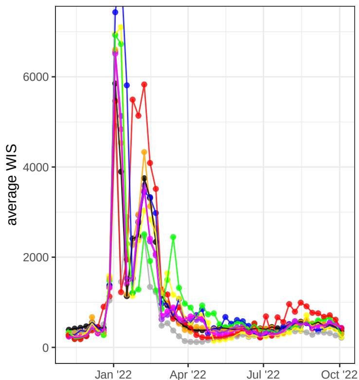
95% coverage (1 week)
