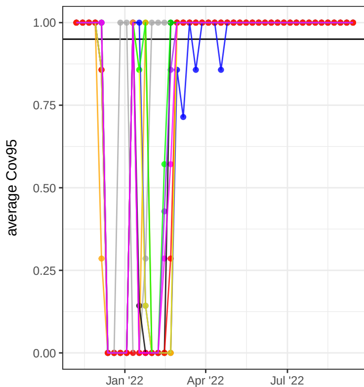
95% coverage (4 week)
