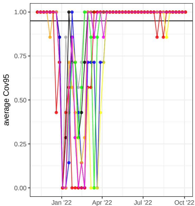
95% coverage (1 week)
