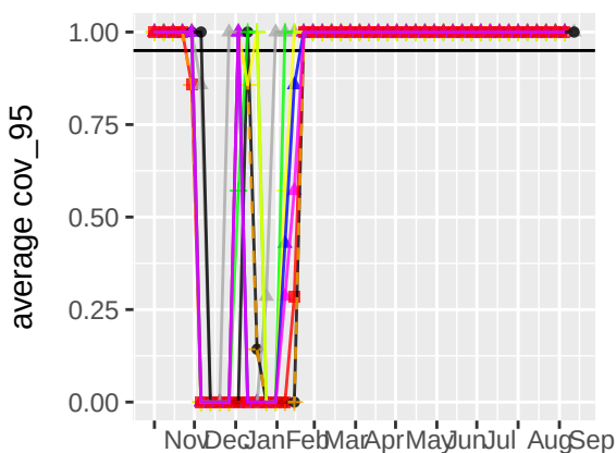
95% coverage (4 week)
