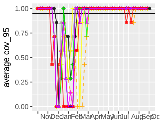
95% coverage (1 week)
