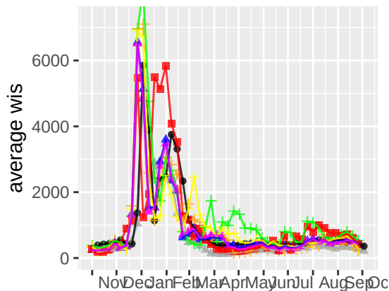
95% coverage (1 week)
