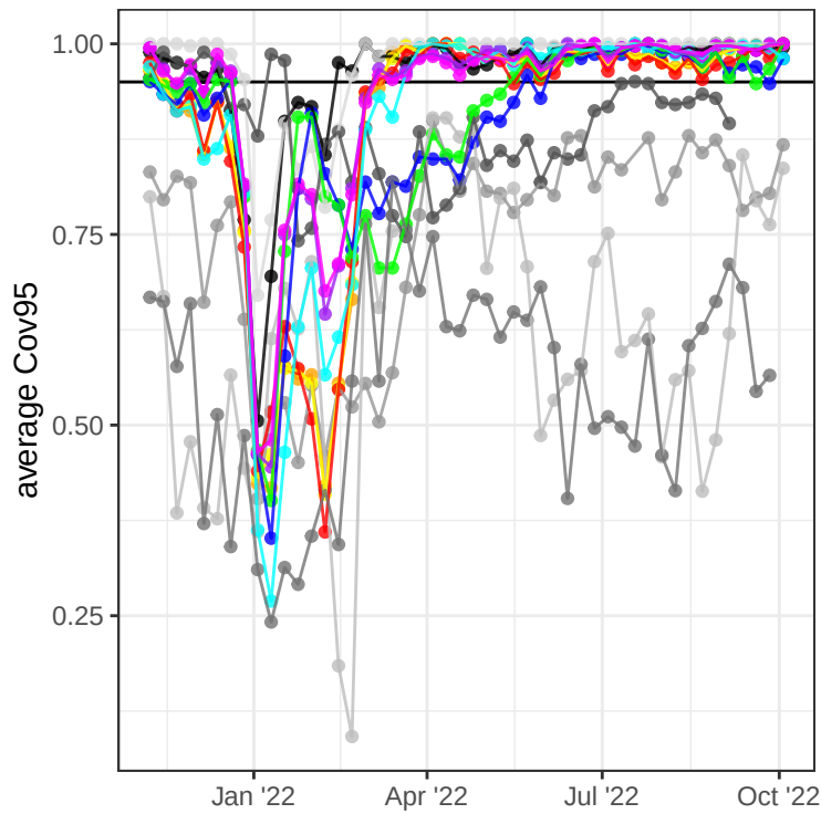
95% coverage (1 week)
