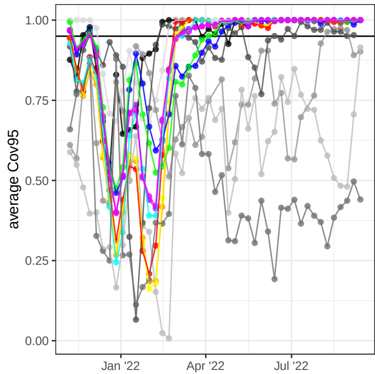
95% coverage (4 week)
