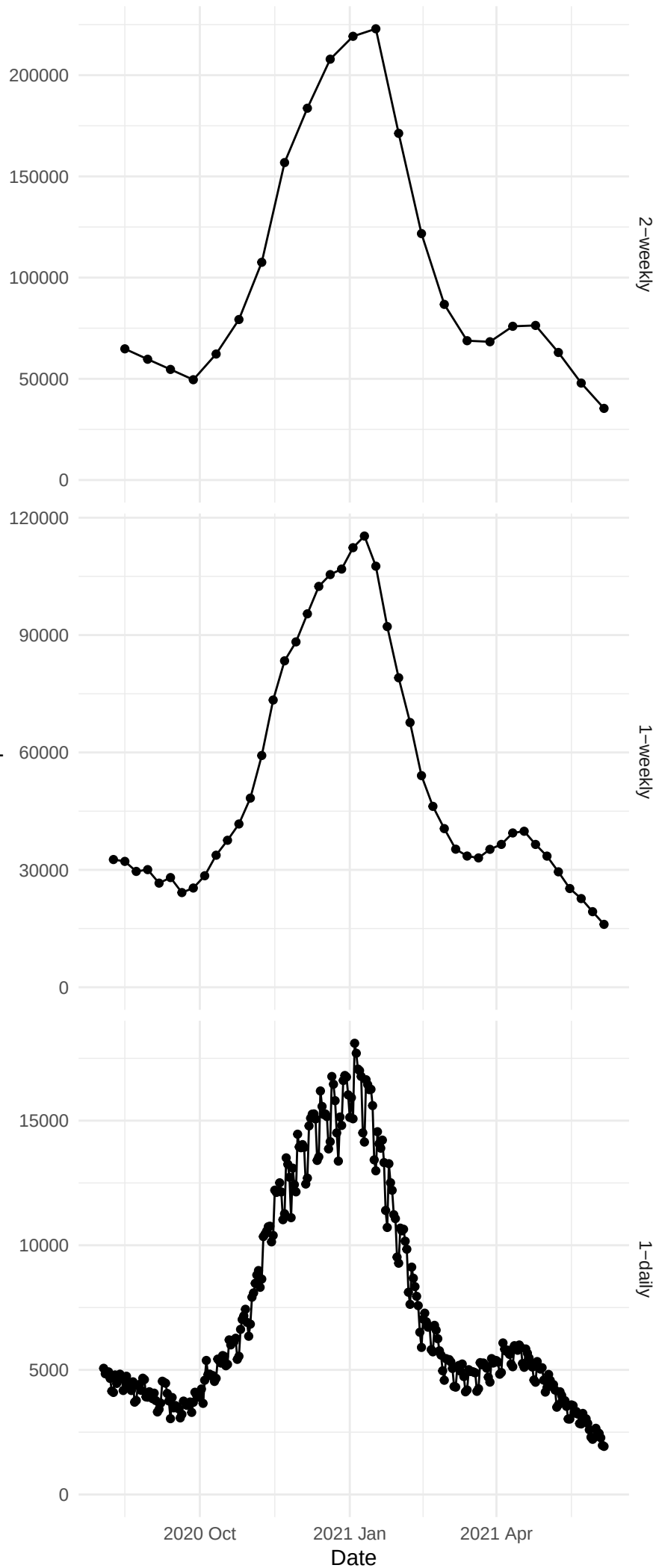
Aggregate Data
