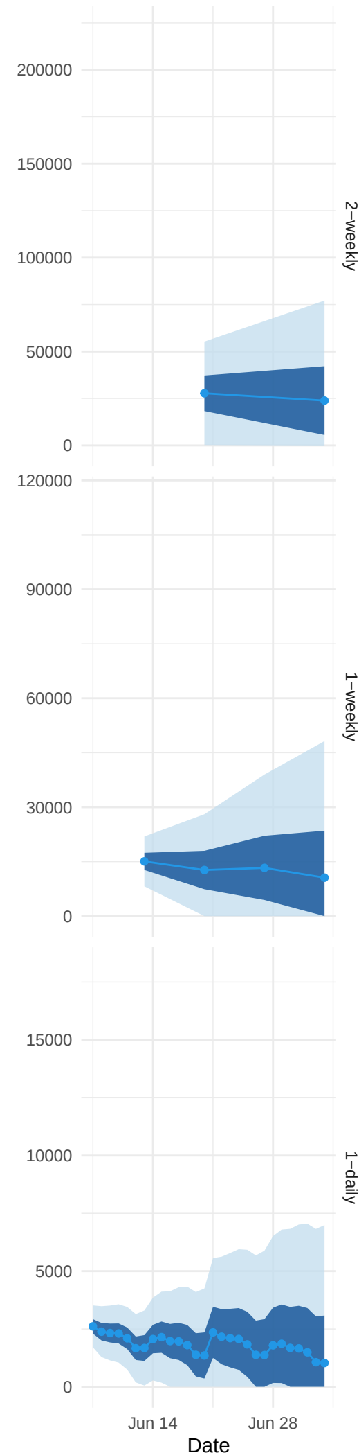
Reconcile Forecasts
