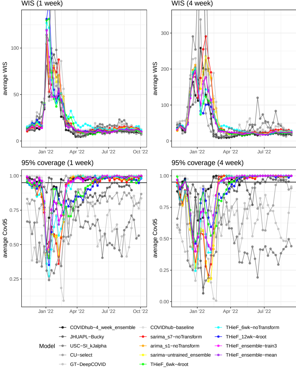
Figure 6: Average h -week ahead WIS and 95% PI coverage plotted by forecast week during the testing phase for each model for averaged states. The plotted WIS values generally follow the shape of the incident hospitalization truth data, with greater values occurring during times of high incidence and rapid change. The 95% coverage rates tend to follow a vertically flipped transformation of the truth data, with below-nominal coverage rates observed during times of high incidence and rapid change.
