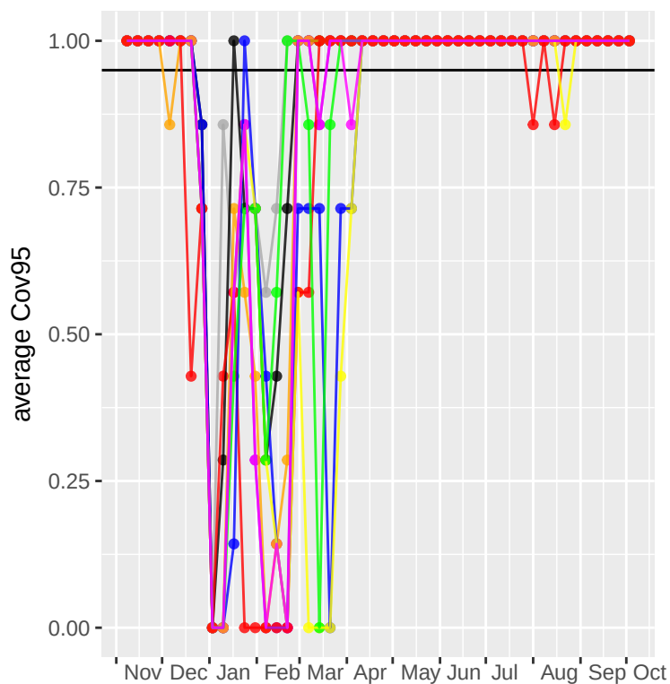
95% coverage (1 week)
