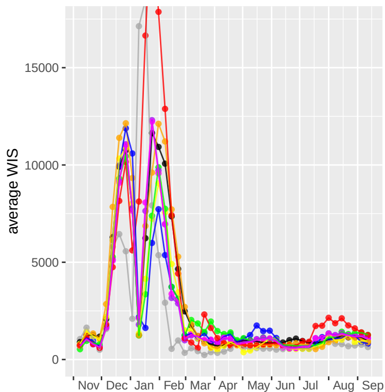
95% coverage (4 week)
