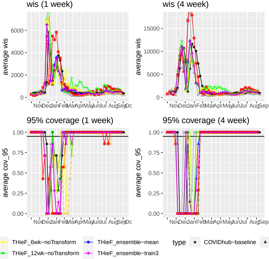
Figure 1.5. Average h-week ahead WIS and 95% PI coverage for each model for the US national level. Model performance differs from week to week: the WIS is the lowest during weeks with stable and low incident hospitalization values. The THieF-4wk models show the best performance with lower or comparable WIS to the baseline during the majority of the training period with especially good performance for 1-week ahead horizons. Meanwhile, the THieF-12wk showed lower or comparable WIS to the baseline during high incidence and changed points, which have been historically found difficult to forecast accurately. Plots for h-week ahead MAE are not shown due to their similarity to the WIS plots. All THieF models show very variable coverage rates, especially for a 1 week ahead horizon, only the models without a data transformation showing stable coverage starting around February 2021.
