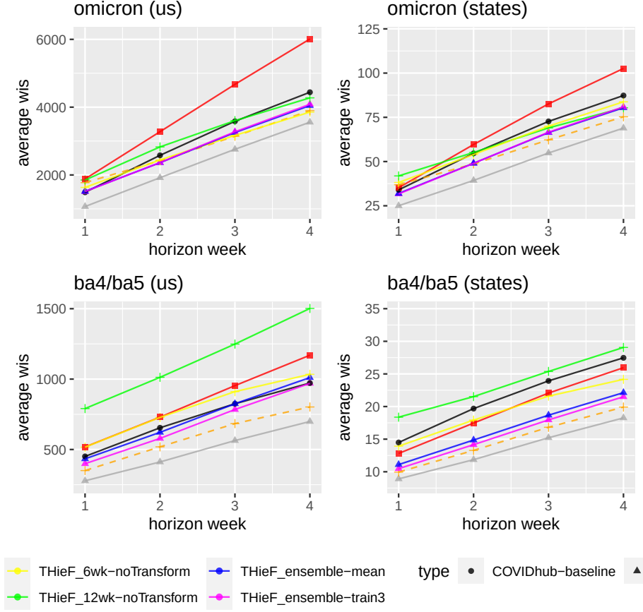
Figure 1.3. Average WIS by the horizon week and pandemic wave for each model for the US national level and the states level. The figures show similar trends in WIS when forecasts are stratified by horizon week and pandemic wave compared to being stratified only across horizon week. Again, all models show worse performance relative to the baseline at the 1-week ahead horizon likely due to being overconfident at this horizon. Model performance is more similar among the top four models during the Alpha wave compared to during the Winter21 wave. Notably, although the THieF-4wk-4root models largely show the lowest WIS, longer horizons during the Winter21 wave saw better performance by the poor-performing THieF-12wk models. Plots for average MAE are not shown due to their similarity to the average WIS plots.
