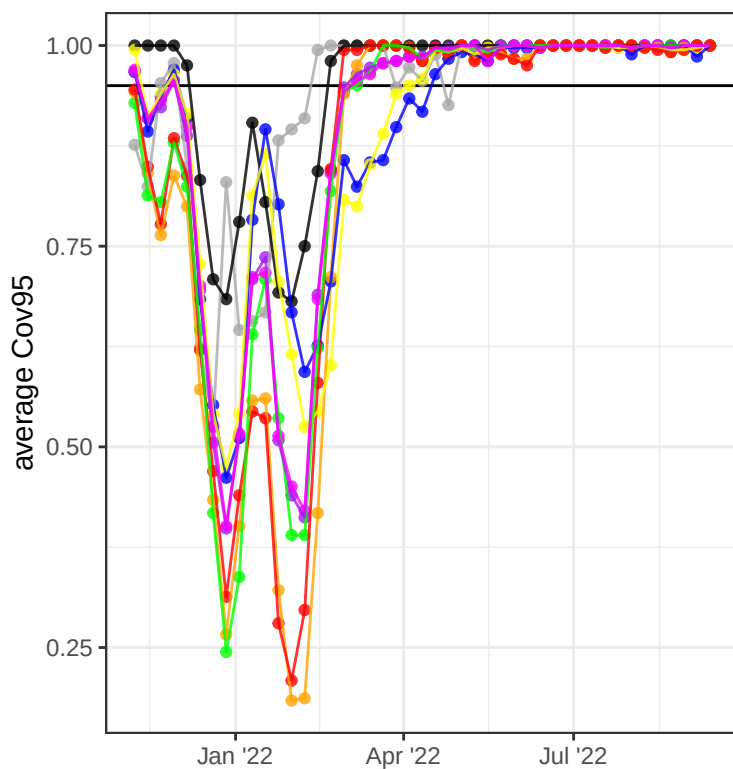
95% coverage (4 week)
