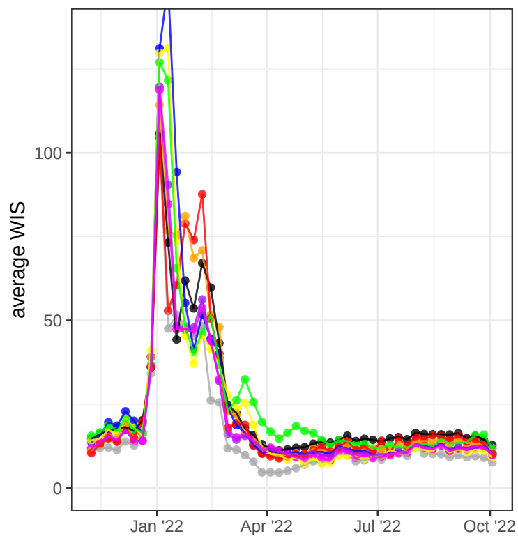
95% coverage (1 week)
