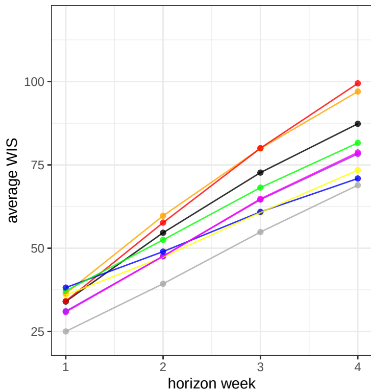
BA.4/BA.5 (States)
