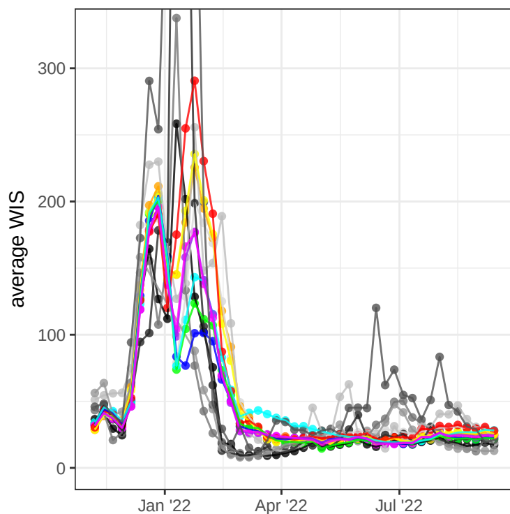
95% coverage (4 week)
