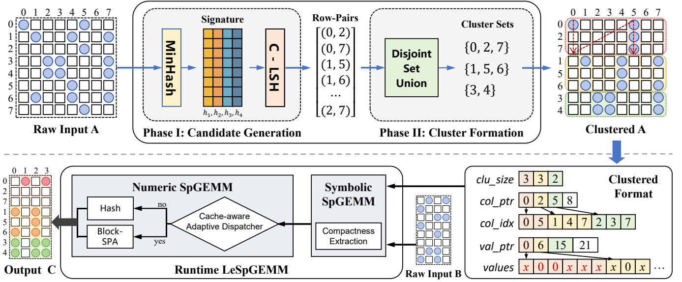
Fig. 4: An overview of LeSpGEMM, where the upper half performs row-clustering preprocessing on the sparse input A , and the lower half shows the runtime execution of LeSpGEMM computing C = AB .
