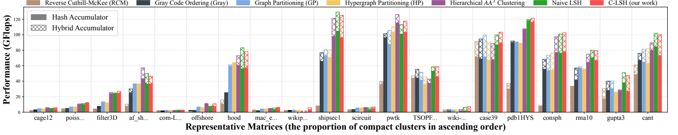
Fig. 10: The ablation study across several reordering algorithms with hash and hybrid accumulators on AMD EPYC 7C13.
