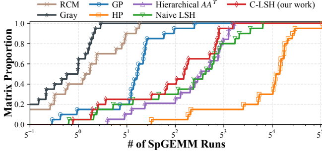
Fig. 11: The time overhead of reordering methods.
