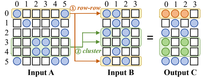
Fig. 2: An example of SpGEMM: ① the row-row workflow of Gustavson’s algorithm; and ② its cluster-wise variation.
