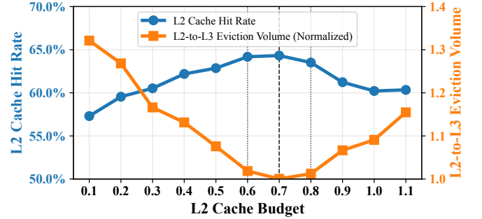
Fig. 8: L2 cache hit rate and normalized L2-to-L3 eviction volume versus the L2 cache budget on Intel Xeon 5120 CPU.
