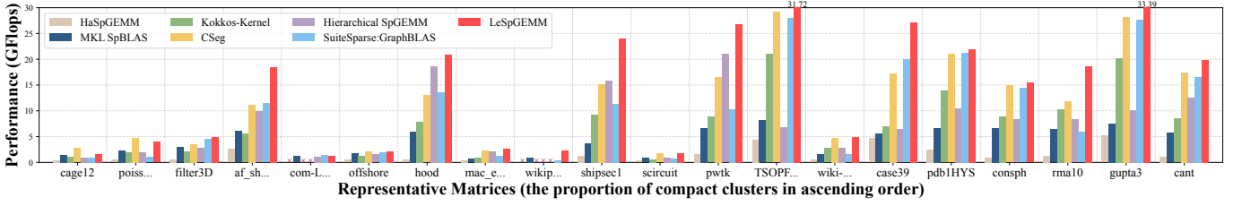
Fig. 9: A double-precision performance comparison on 20 representative matrices on Intel Xeon 5120 CPU.
