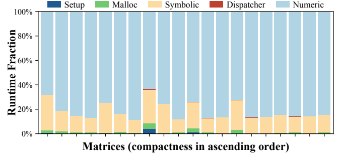
Fig. 13: The runtime breakdown of LeSpGEMM.
