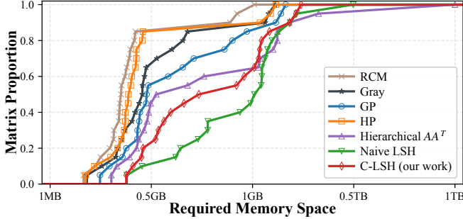
Fig. 12: The memory consumption of reordering methods.
