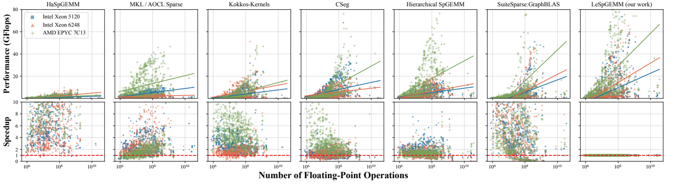
Fig. 6: Performance comparison of LeSpGEMM against six state-of-the-art SpGEMM algorithms on Intel Xeon 5120, Xeon 6248 and AMD EPYC 7C13 processors. The top row presents double precision performance of C = A^2 along with linear regression fits, while the bottom row shows the corresponding speedups of LeSpGEMM over competing methods.
