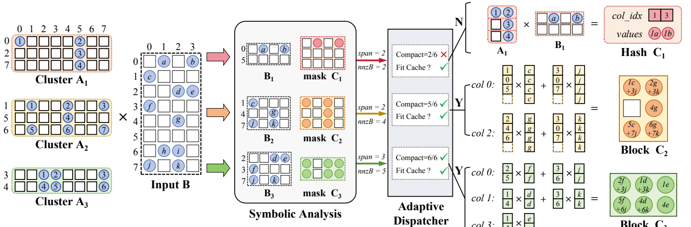
Fig. 5: An example of runtime LeSpGEMM execution. First, during the symbolic analysis, we can obtain the number of corresponding elements in B and the structure of C . Next, by analyzing cache utilization and compactness through a cache-aware adaptive dispatcher, LeSpGEMM calls different accumulators to complete the accumulations. In this example, we assume the L2 cache budget L2\_bg is 1MB , and the compactness threshold \tau is 0.5 .
