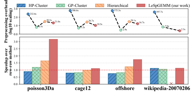
Fig. 1: A brief observation on the performance improvement and preprocessing overhead of existing SpGEMM algorithms.
