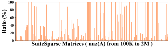
Fig. 3: Ratio of compact clusters ( compactness > 50\% ) in resulting matrix C when computing C = AA .
