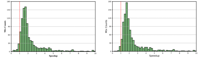
(a) Predicted algorithms by SSpMV (b) Hand-pick best SpMV algorithms Fig. 8. Speedup Distribution of isolated SpMV performance over Intel MKL.
