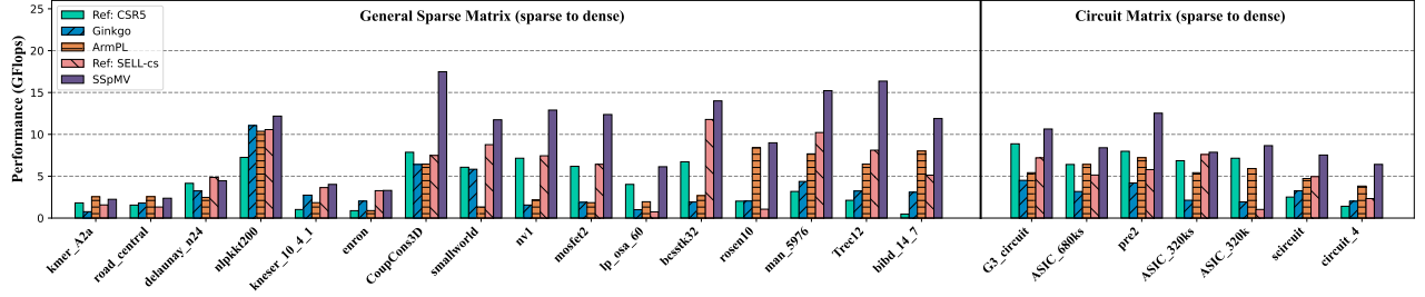
Fig. 10. Performance comparison with other libraries on Huawei Kunpeng 920 processors.
