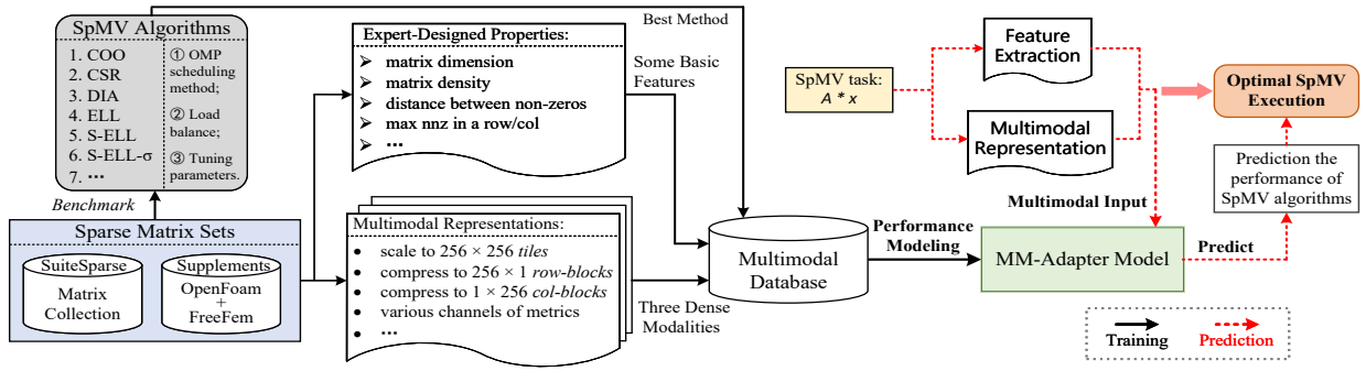
Fig. 4. Overview of the Sparsity-aware SpMV framework.
