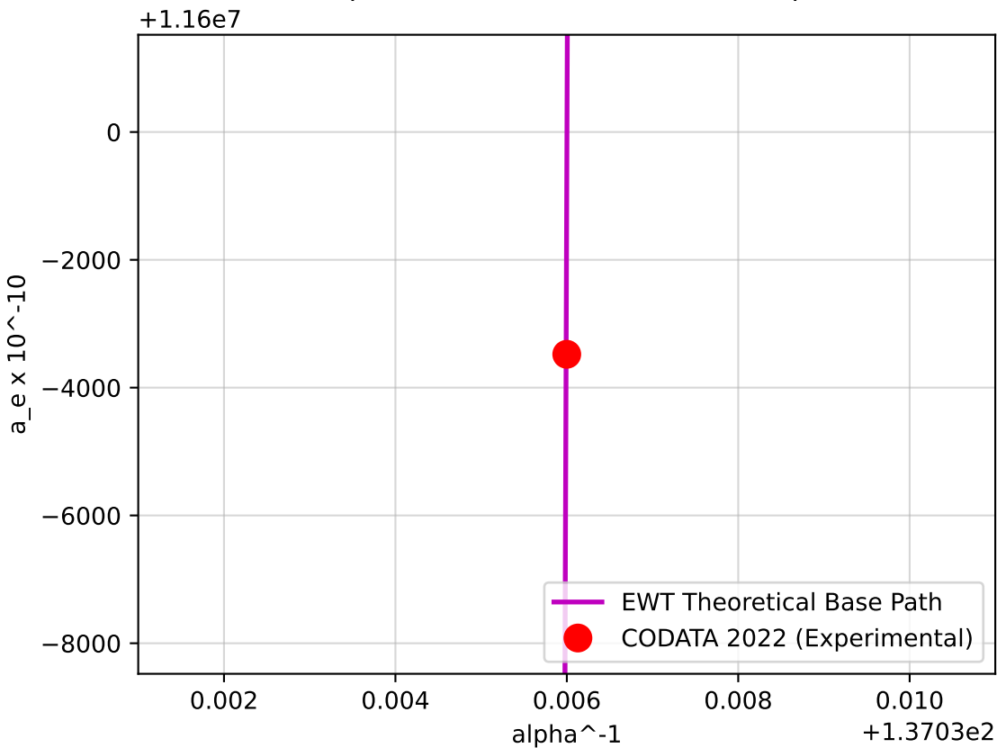
Phase Space: Electron AMM Base vs Alpha -1
