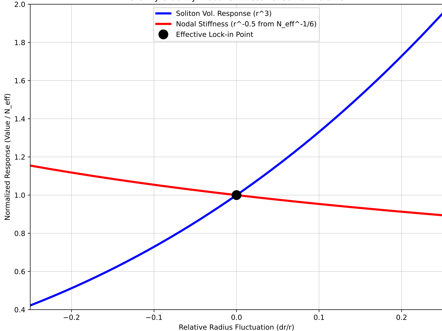
Gravity Stability: Nodal Stiffness vs. Soliton Volume
