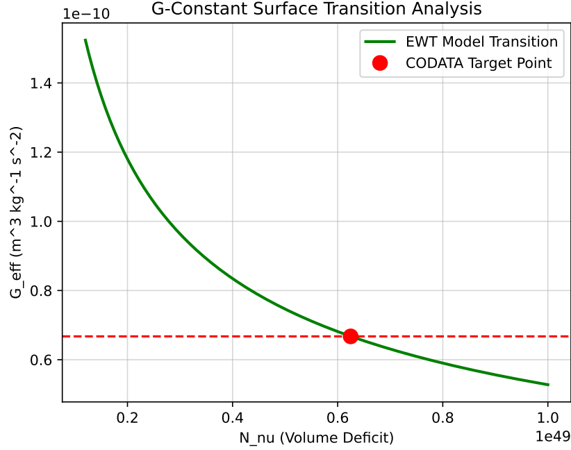
Figure 9: Analysis of the G-constant surface transition. The green curve illustrates the evolution of G as a function of the effective volume deficit N_{\nu} . The red intersection point marks the deterministic alignment with G_{\text{CODATA}} at the calculated N_{\nu,\text{eff}} .
