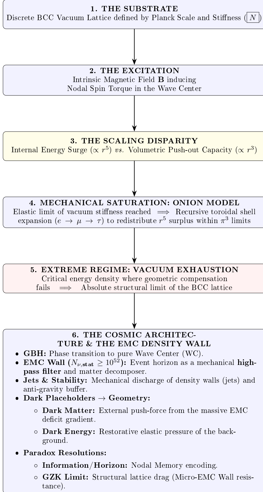
Figure 19: The hierarchical emergence of physical constants and cosmic structures within the EWT framework.
