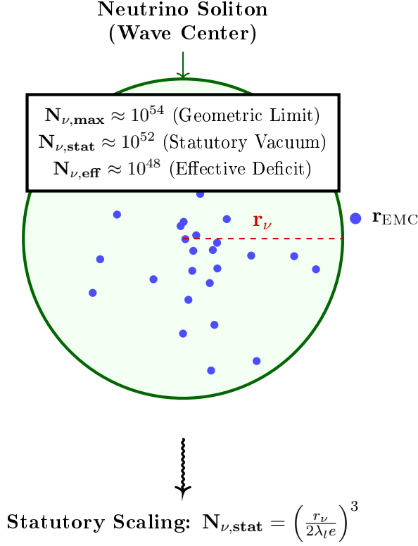
Figure 4: Hierarchical Topology of the Neutrino Soliton. The model establishes a clear dilution gradient from the theoretical geometric limit ( N_{\nu,\max} ) to the statutory vacuum density ( N_{\nu,\text{stat}} ). The final effective volume deficit ( N_{\nu,\text{eff}} \approx 6.25 \times 10^{48} ) represents the integrated packing density of the wave center, which acts as the source of the gravitational potential. This hierarchical structure confirms that gravity emerges from the residual geometric displacement within the high-density EMC medium.
