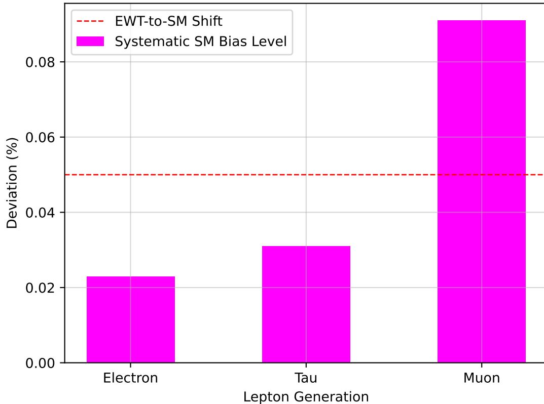
Lepton Error Spectrum: EWT Geometry vs SM Interpretation
