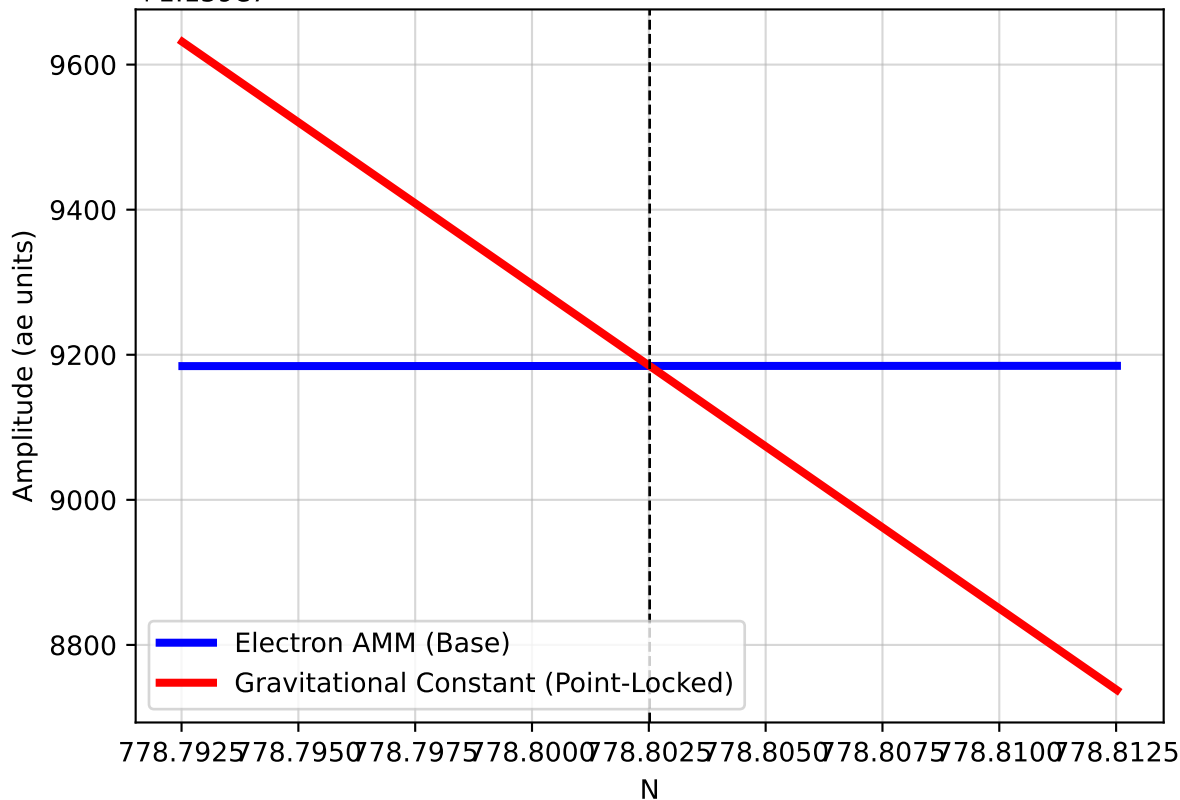
EWT Unified Point-Lock: G anchored to Electron AMM at N_{\text{geom}} + 1.159e7
