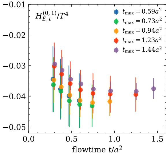
two-mass fits
