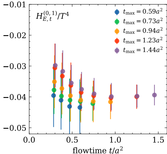
one-mass fits
