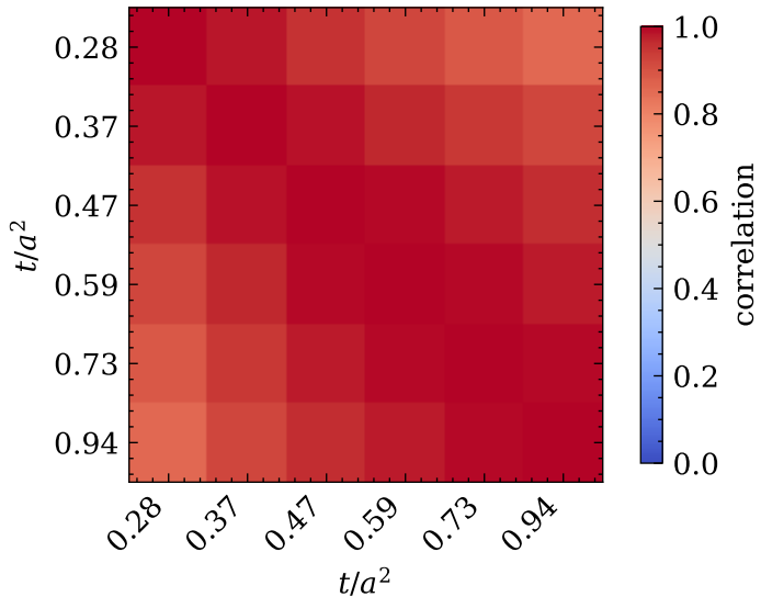
Correlations of H_{E,t}^{(0,1)} in t (two-mass fit)
