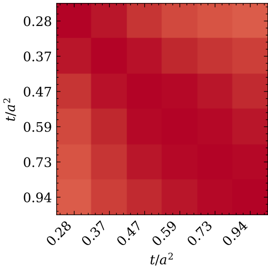
Correlations of H_{E,t}^{(0,1)} in t (one-mass fit)
