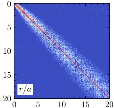
mode 1, t = 0.73a^2
