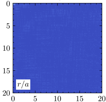
mode 0 vs 1, t = 0.73a^2
