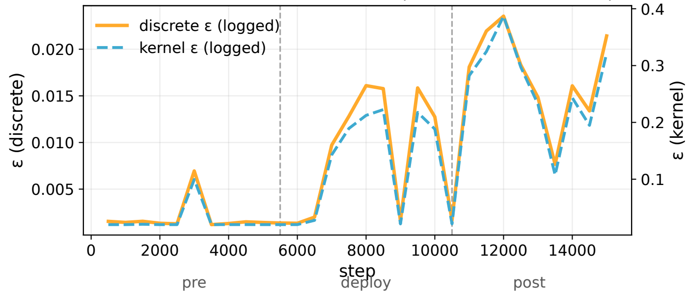
Residual-OI \varepsilon : discrete vs kernel (calibration residual r0)
