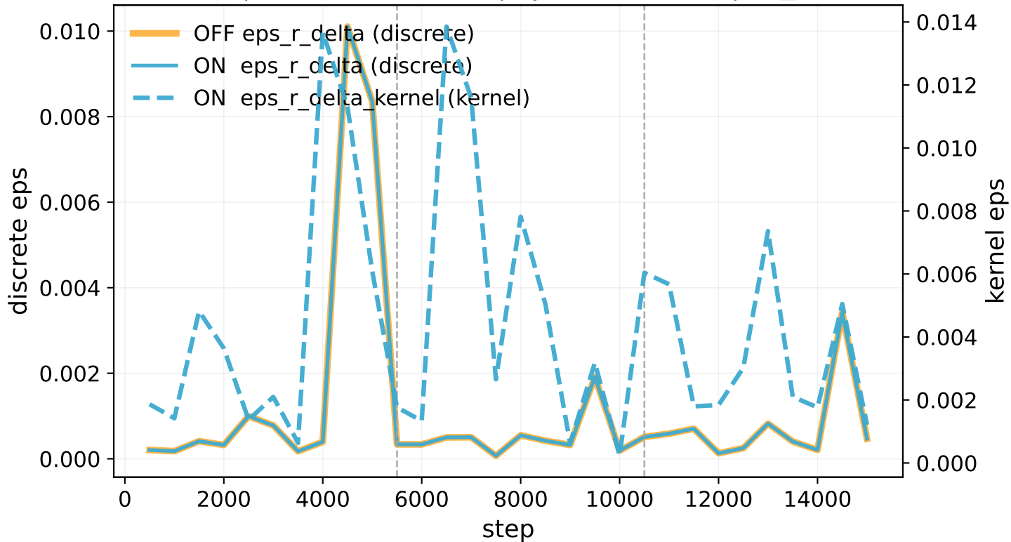
Residual pre-OL eps: discrete vs kernel (TE residual post_delta)
