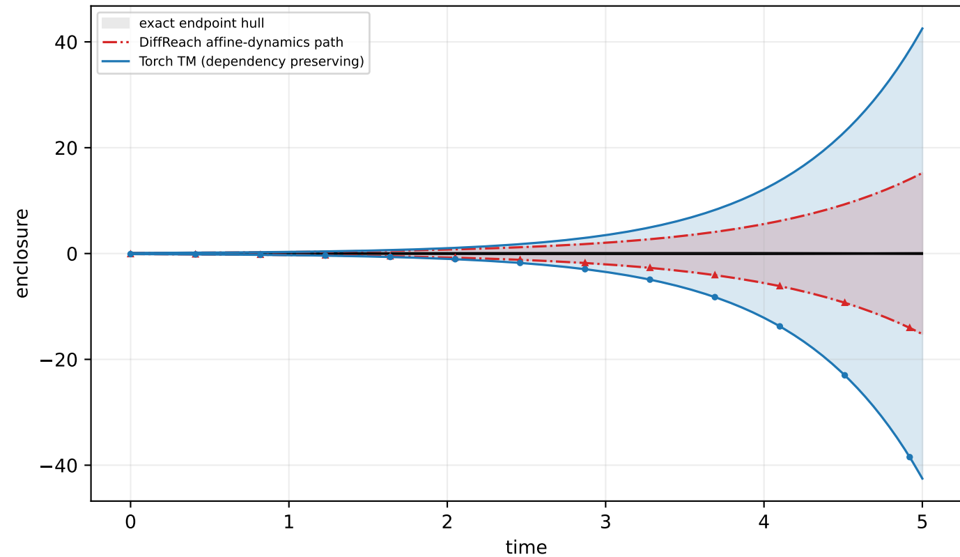
harmonic: state 0, h=0.01 , T=5 (primary)
