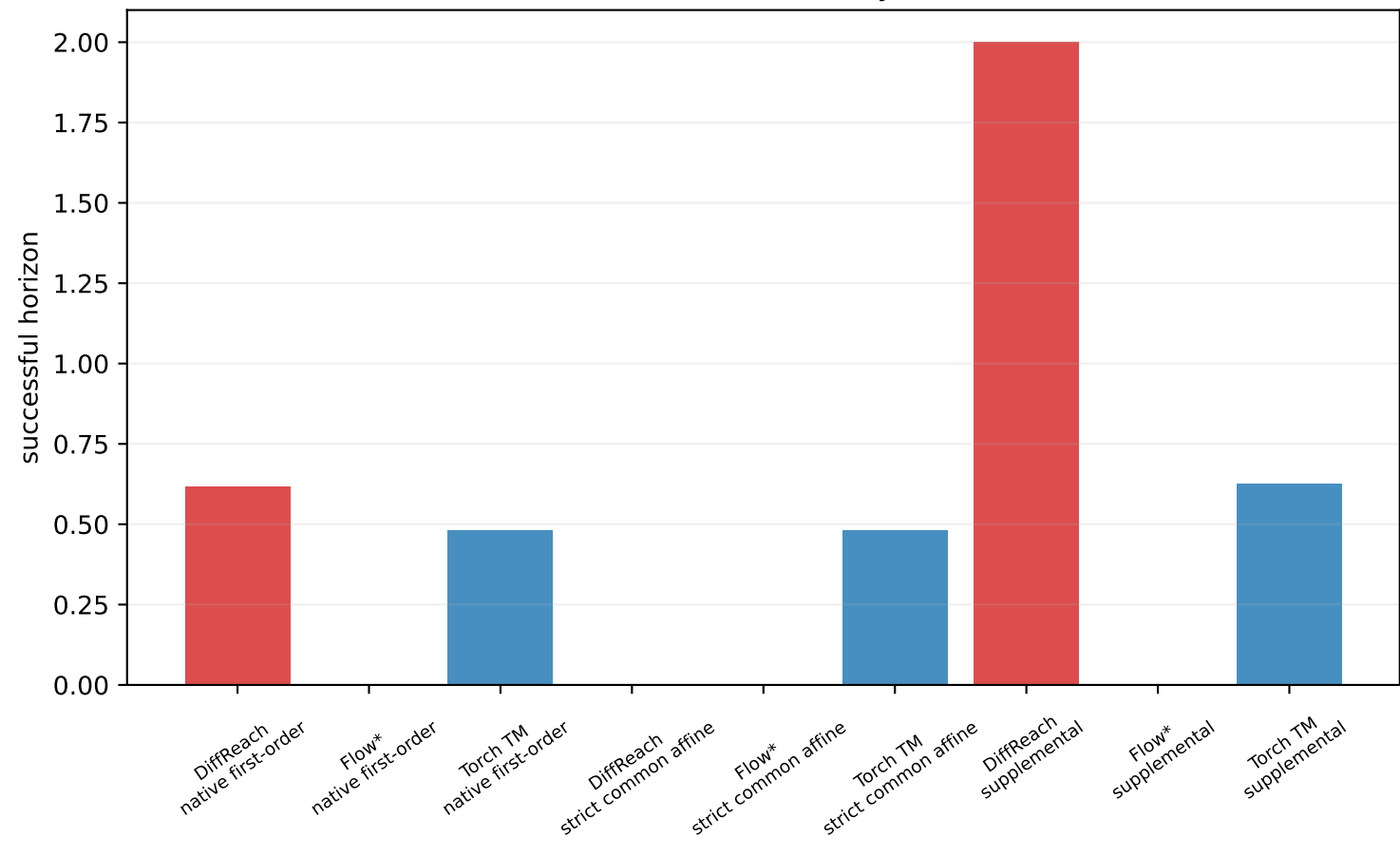
Van der Pol: maximum successfully validated horizon
