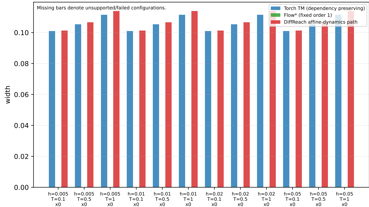
riccati: final endpoint widths (primary)
