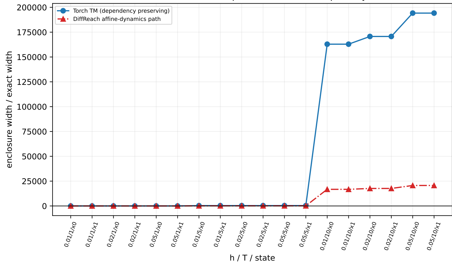
harmonic: exact endpoint inflation ratio (primary)
