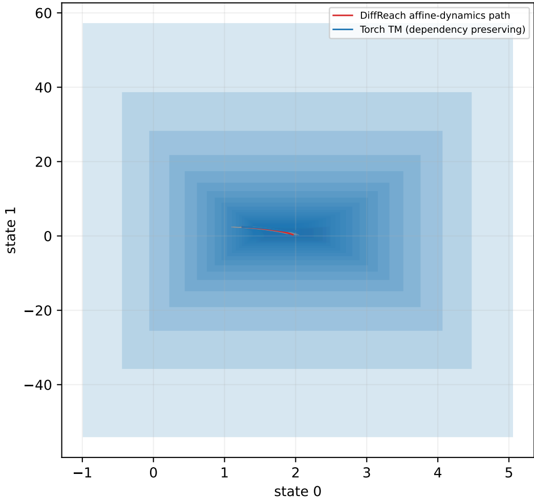
van_der_pol: phase-plane enclosures, h=0.01 , T=0.5 (primary)
