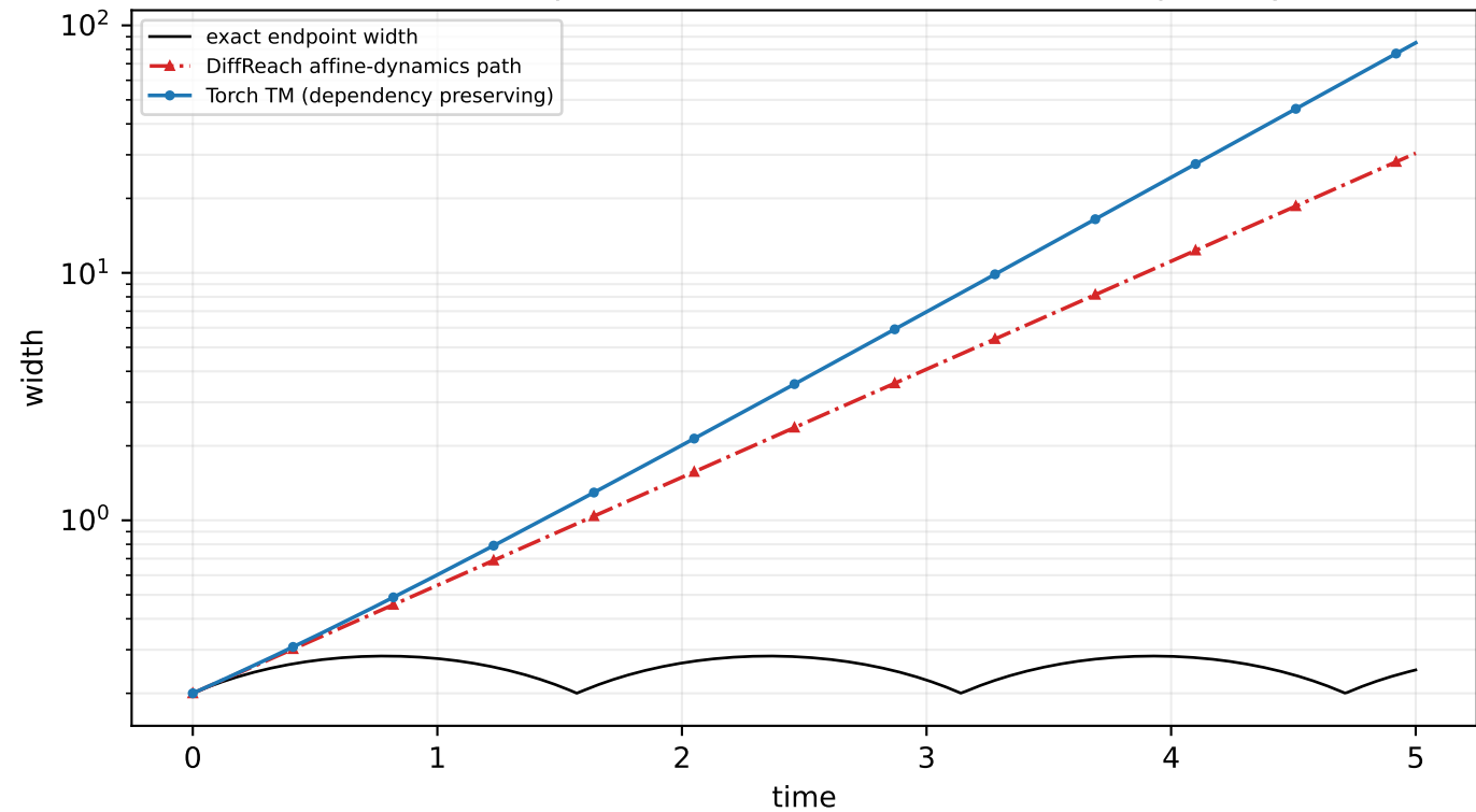
harmonic: endpoint width, state 0, h=0.01 , T=5 (primary)
