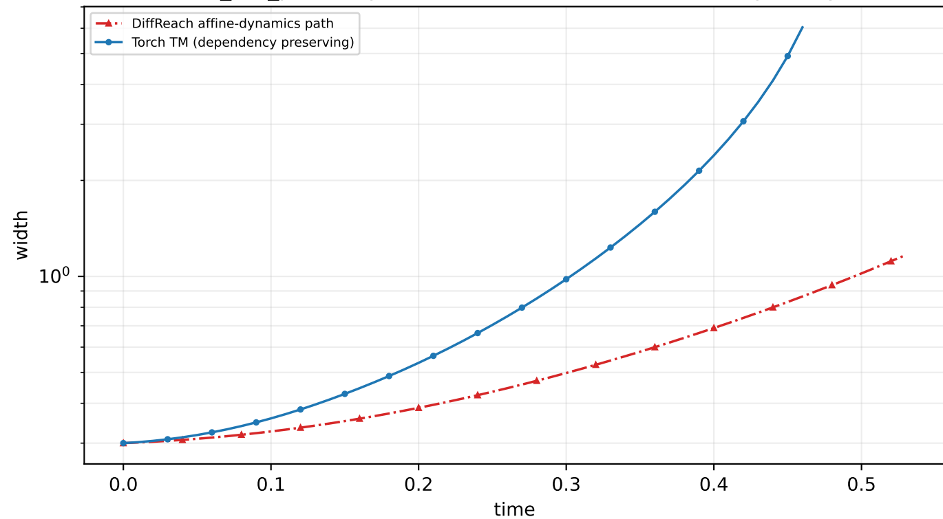
van_der_pol: endpoint width, state 0, h=0.01 , T=1 (primary)
