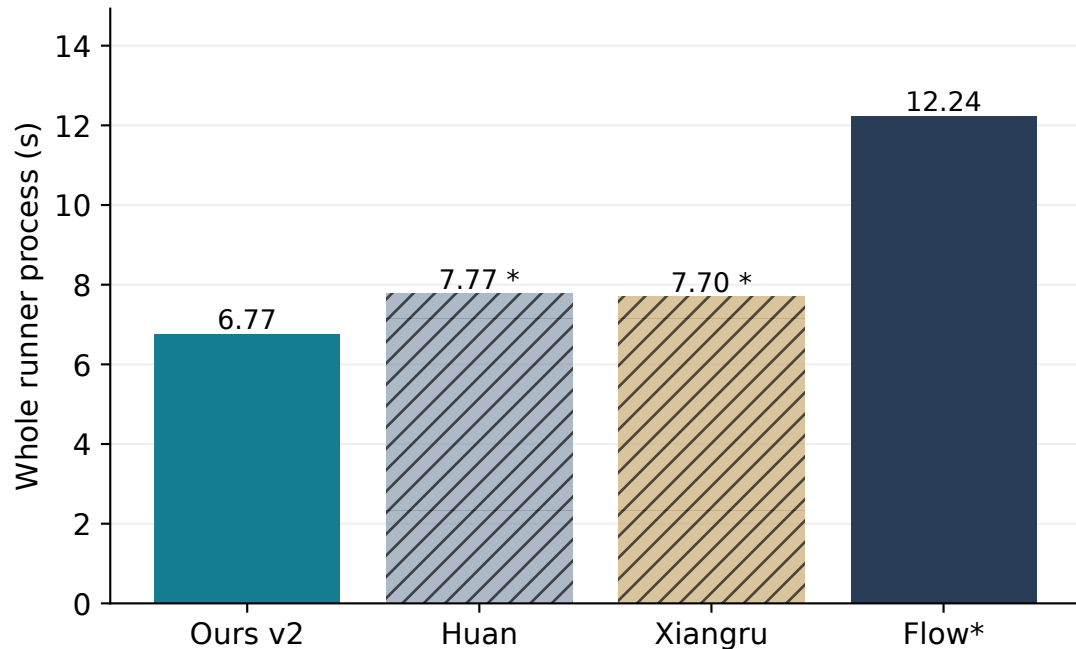
TORA: B12 × 200
