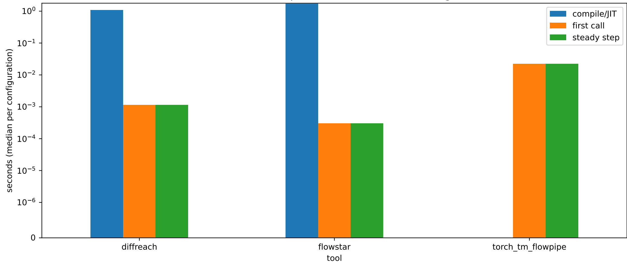
Runtime decomposition (not a combined ranking)
