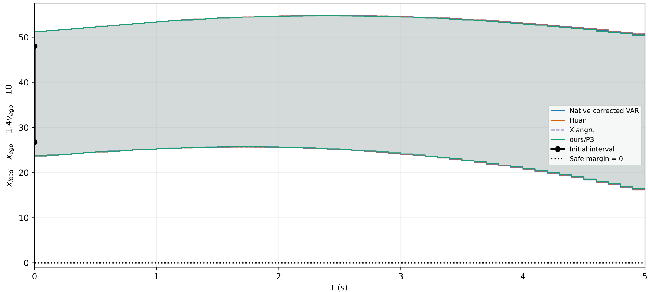
2026 ACC participant-order variant, four methods, T=5, full initial box — saved tube
