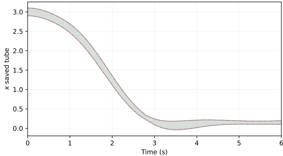
Robust: x
