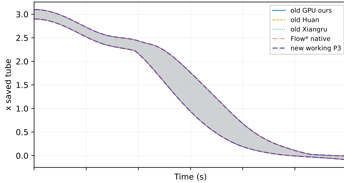
Robust: x
