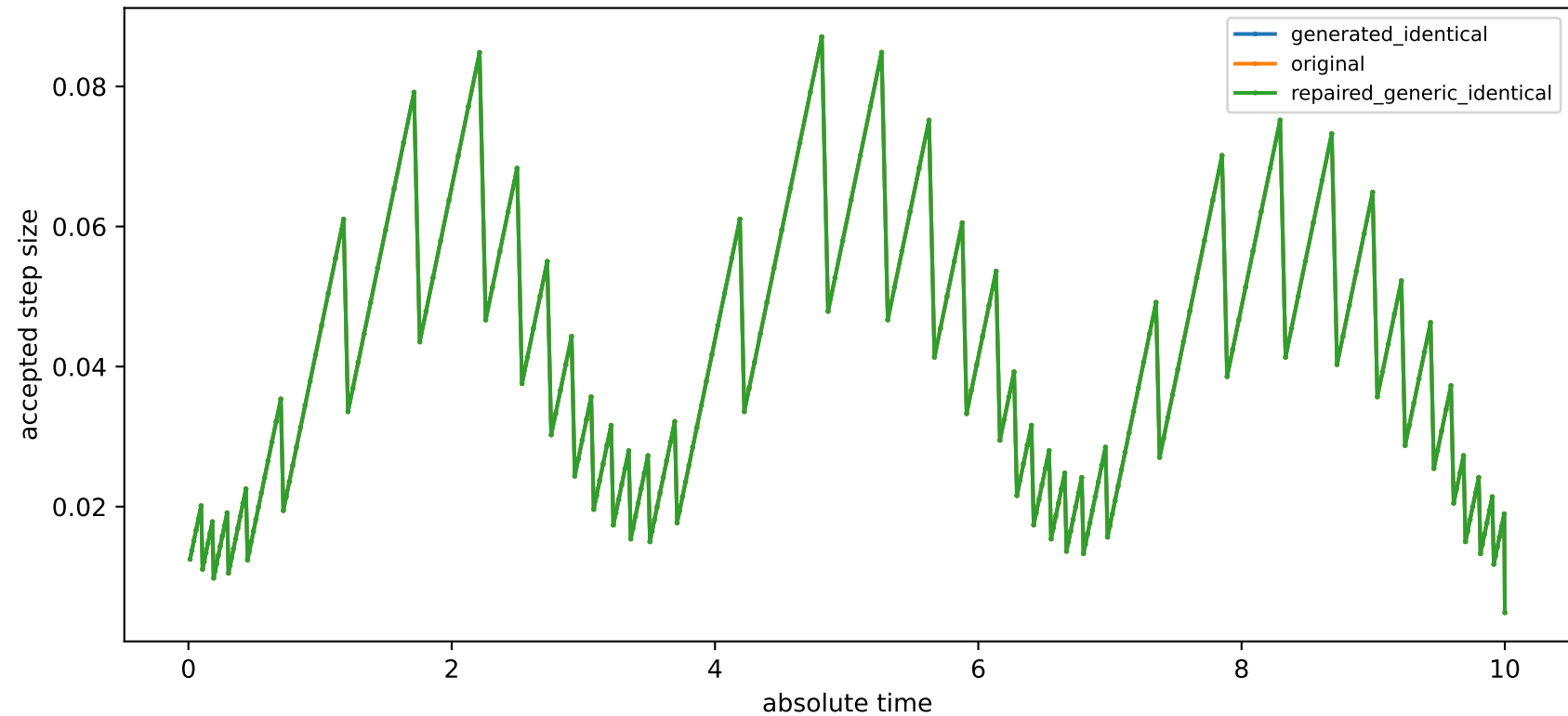
Flow* original benchmark and identical-settings harnesses
