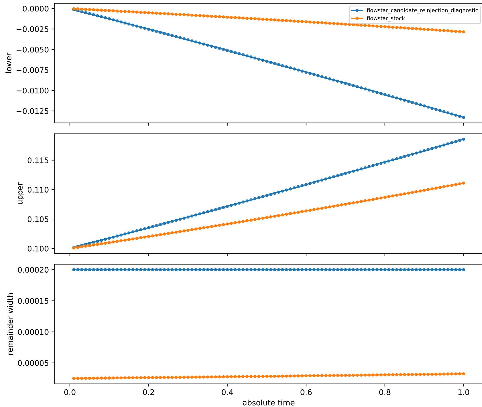
Flow* stock versus candidate-reinjection diagnostic
